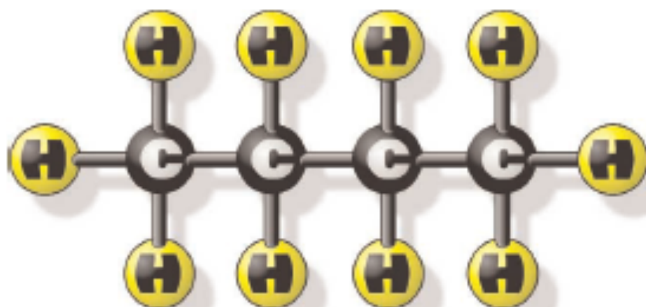
Butane ( \text{C}_4\text{H}_{10} )
